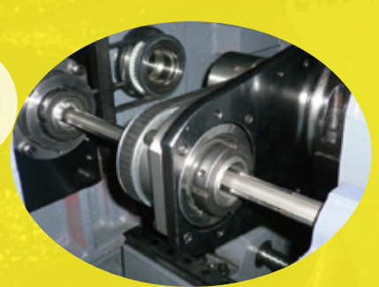
主軸同步迴轉導套 Synchronous rotary guide bushing
