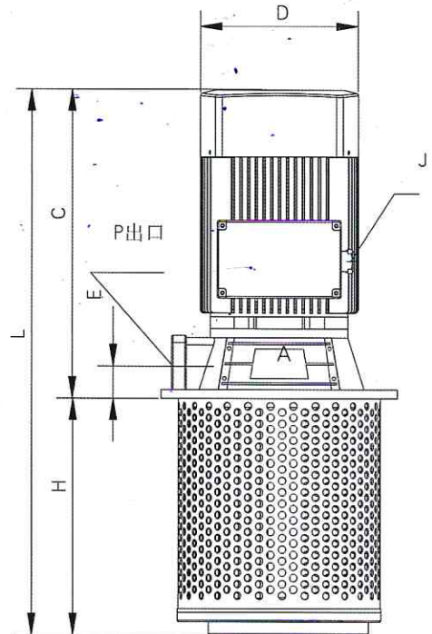
外形图 Appearance in figure
